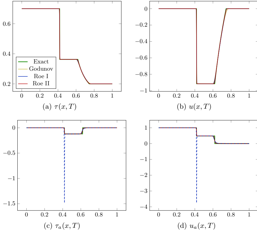
Figure 3.9 – Classical finite volume schemes.
