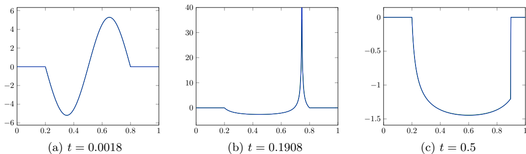
Figure 2.15 – Sensitivity solution for the problem with continuous i.c. with correction, a = x_c .
