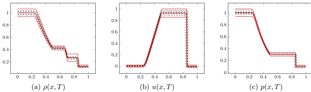
Figure 4.18 – SA approach with correction, anti-diffusive scheme. Average and the average plus and minus twice the standard deviation in red. Five samples in black dashed lines.
