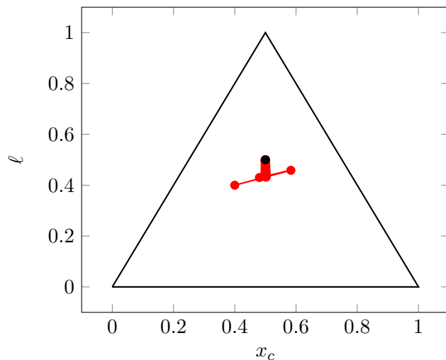
Figure 5.17 – Optimization algorithm steps for the isentropic transonic case, \mathbf{a} = (x_c, \ell) .
