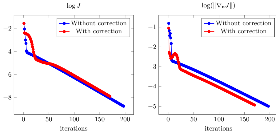
Figure 5.15 – Value of the cost functional and norm of its gradient with respect to iterations in a semilogarithmic scale - shocked flow case, \mathbf{a} = (A, \ell) .
