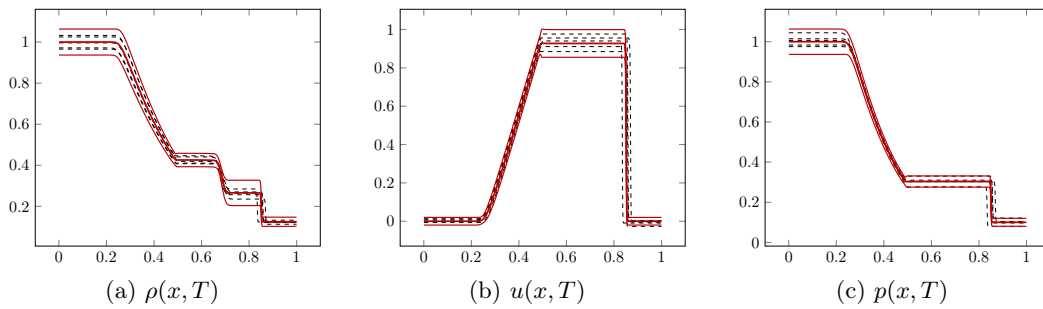
Figure 4.17 – SA approach with correction. Average and the average plus and minus twice the standard deviation in red. Five samples in black dashed lines.
